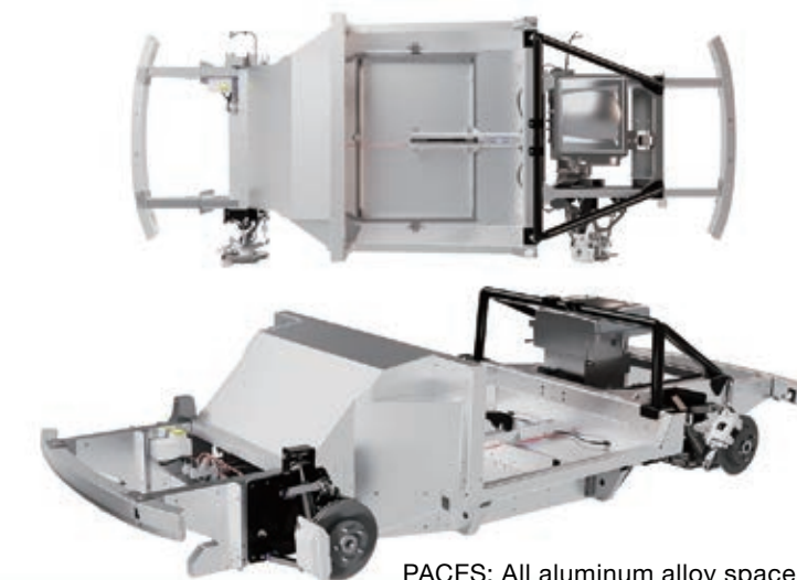
PACES: All aluminum alloy space frame
